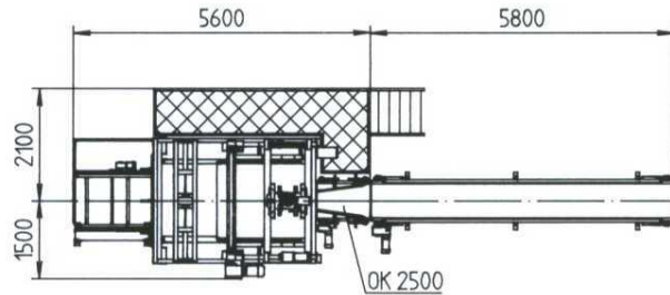
Top view of PIKOMAT HDQ-Compact
